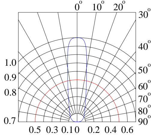
Radiation Diagram
