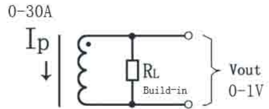
Voltage output type
