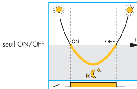
TYPE 11.41 RELAIS CREPUSCULAIRE "HYSTERESIS ZERO"
