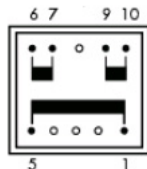
Primary winding
