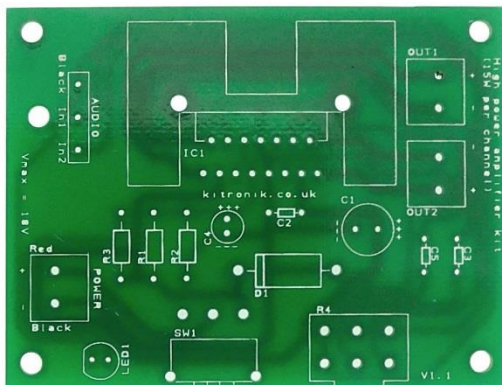
Face composants
